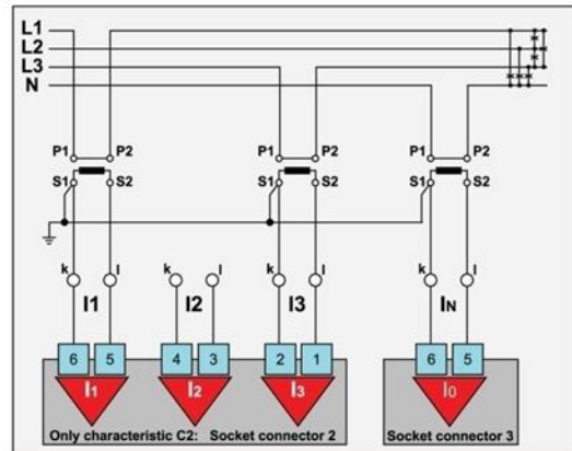
I-configuration 4, 4-phase
