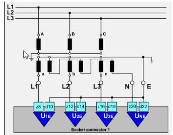
U-configuration 1, 3-phase
