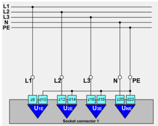
U-configuration 1, 4-phase
