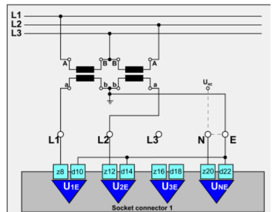
U-configuration 5
