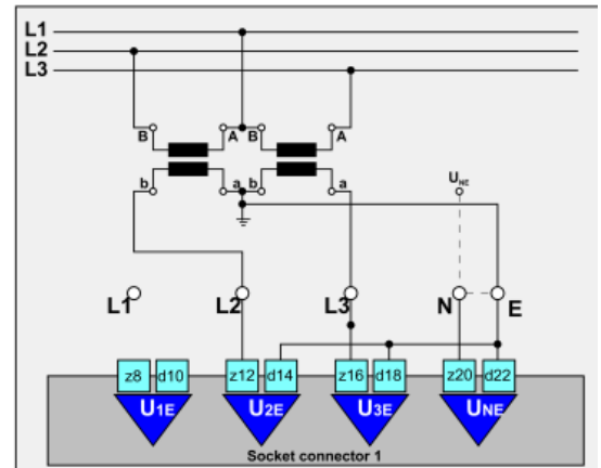
U-configuration 3
