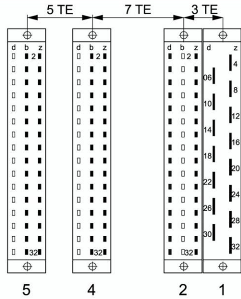
Position of the socket connectors for feature C40... C41
