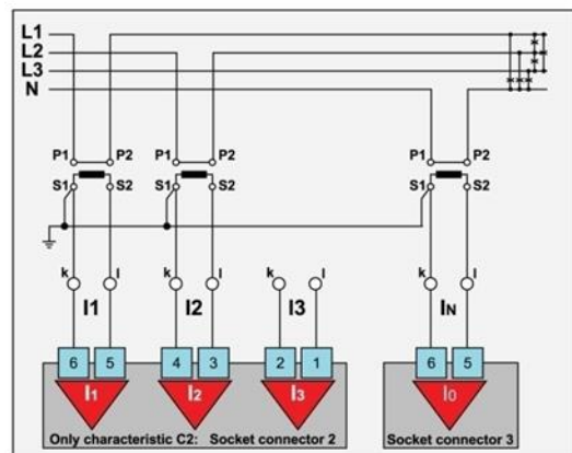
I-configuration 5, 4-phase
