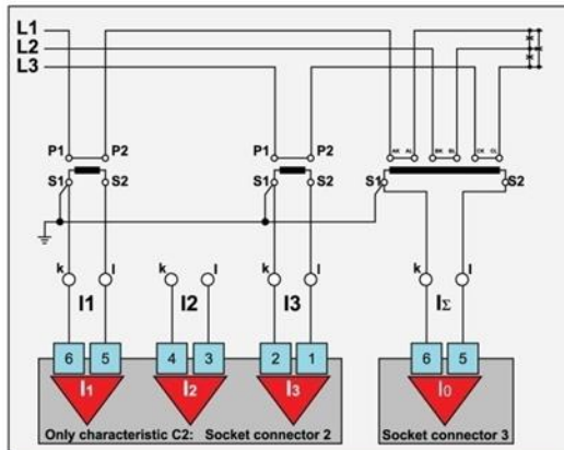
I-configuration 4, 3-phase
