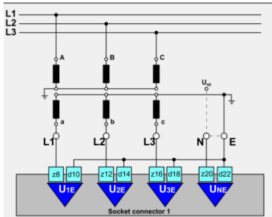
U-configuration 2
