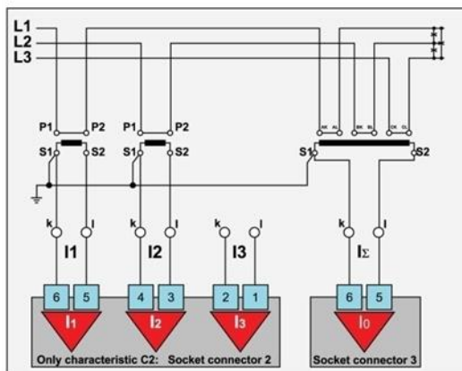
I-configuration 5, 3-phase
