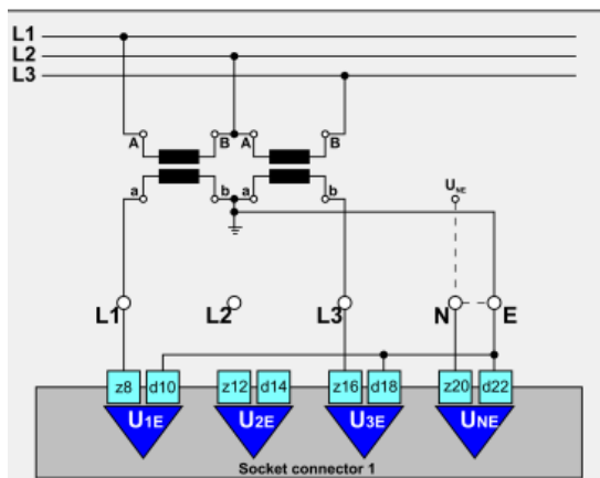
U-configuration 4
